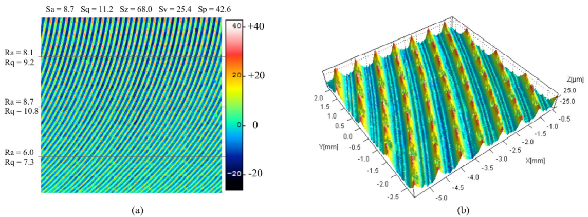
Fig. 3. Quality 2 (rough milling): (a) surface roughness results (in \mu\text{m} ). (b) 3D profilometry of a 5 mm x 5 mm area.
