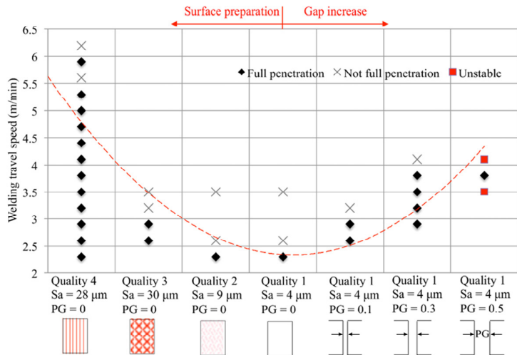
Fig. 6. Comparison of surface preparation and gap increase approaches in terms of welding travel speed and penetration. PG: pre-set gap. Red dashed line: polynomial fit to the maximum travel speeds for full penetration, showing the distribution direction of the experimental points.
