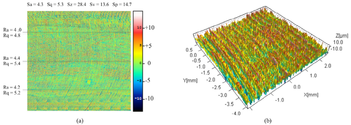
Fig. 2. Quality 1 (industrial milling): (a) surface roughness results (in \mu\text{m} ). (b) 3D profilometry of a 5 mm x 5 mm area.
