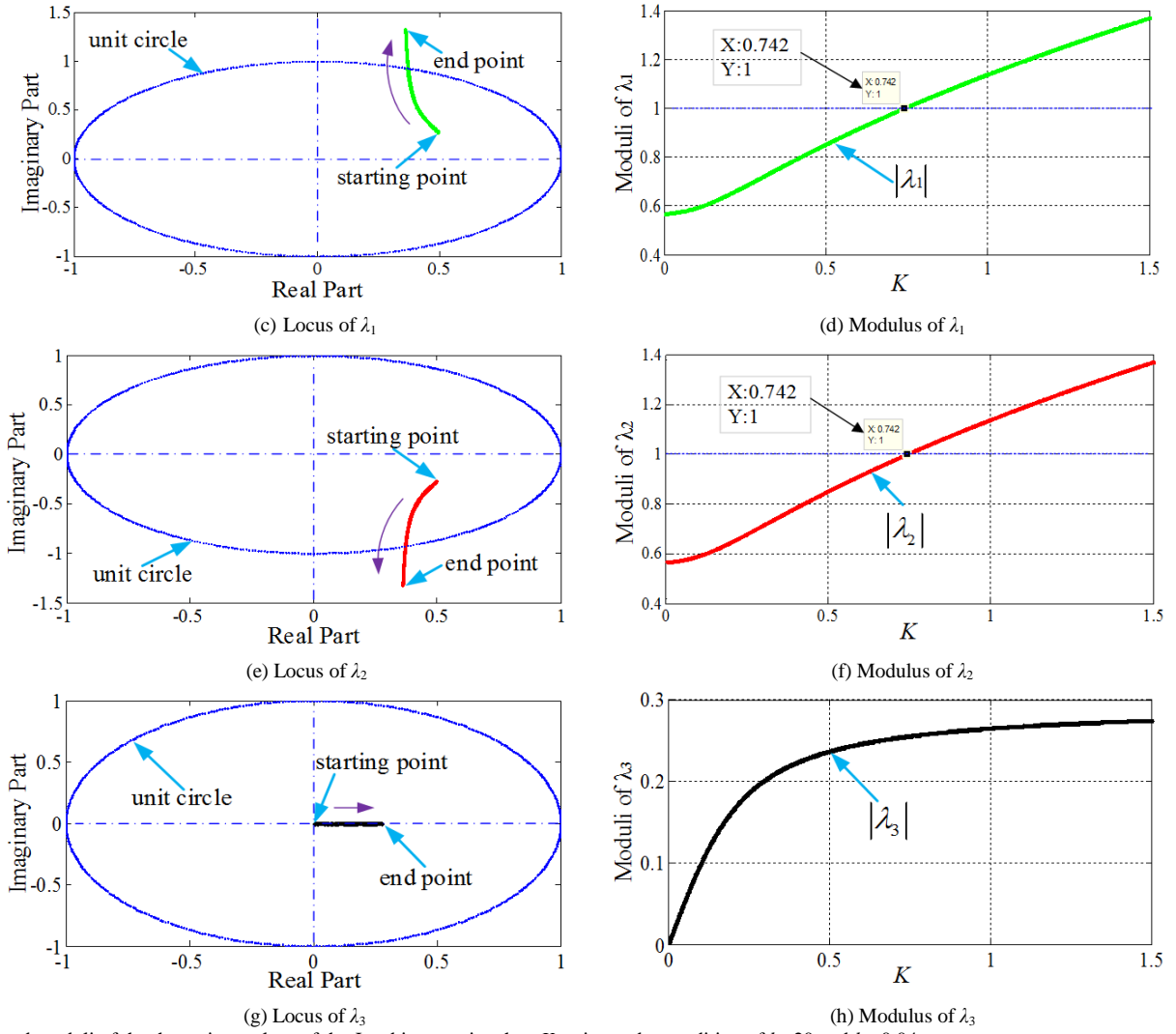
Fig. 12. Loci and moduli of the three eigenvalues of the Jacobian matrix when K varies under condition of k_i=20 and k_p=0.04 .
