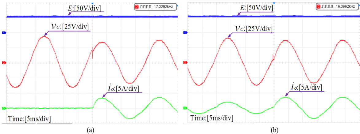
Fig. 20. Transient waveforms under inductive-resistive load condition when k_i=20 , K=0.5 and k_p=0.04 (a) Transient waveforms in response to no load to nominal resistive load step change; (b) Transient waveforms in response to -50% step change of load resistor
