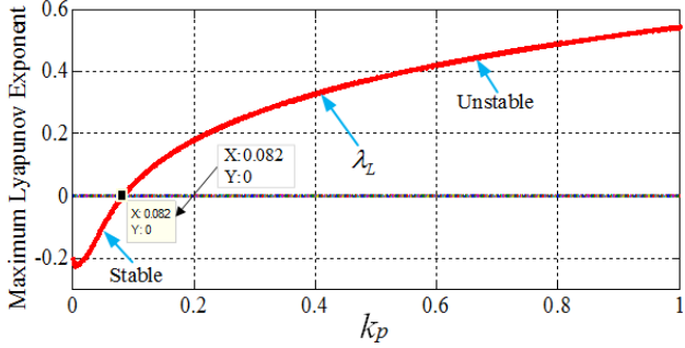
Fig. 9. The maximum Lyapunov exponent spectrum on k_p , under resistive load condition when k_i=20 and K=0.5 .
