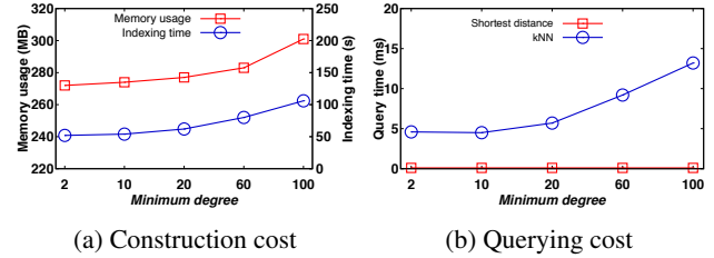
Figure 7: Effect of minimum degree t on VIP-Tree
