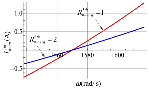
Fig. 10. Relationship of I_{n-oq}^{5th} and \omega with fixed R_{n-virdq}^{5th} (improved ACSC)
