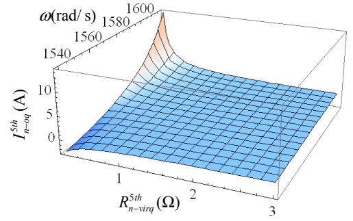
Fig. 9. Relationship of R_{n-virdq}^{5th} , I_{n-oq}^{5th} and \omega (improved ACSC)
