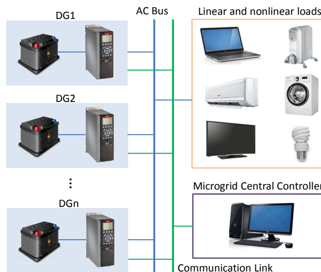
Fig. 1. Overall scheme of an islanded microgrid.
