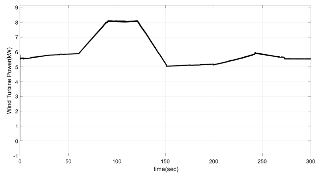
Fig.4. profile of wind turbine power
