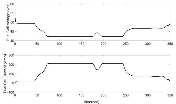
Fig. 5. Variations of fuel cell current and voltage in fuel cell
