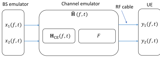
FIGURE 3. A system schematic for 2 \times 2 MIMO in the synthetic MPAC setup.
