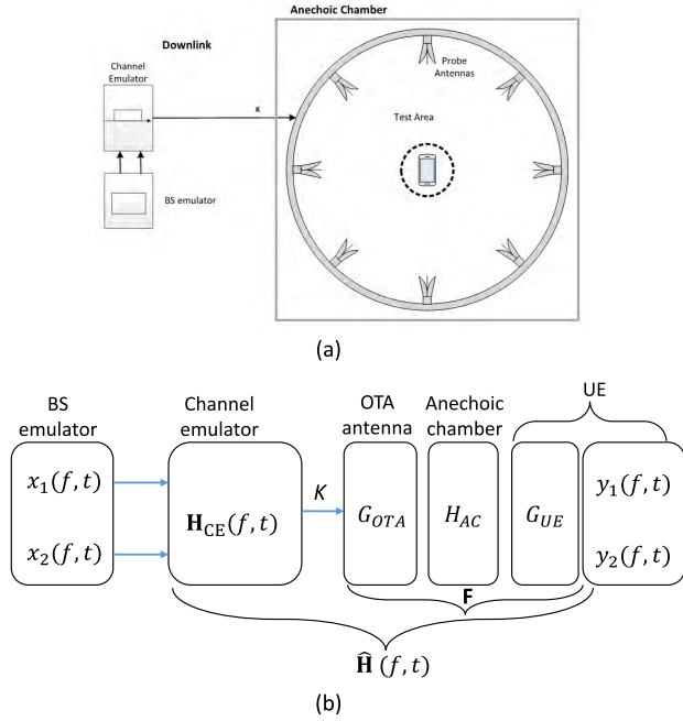
FIGURE 2. (a) A system schematic for 2 \times 2 MIMO in the MPAC setup, and (b) block diagram of the signal model. Note that the uplink is neglected in the top figure for simplicity. G_{OTA} , H_{AC} , and G_{UE} denote the OTA antenna characteristics, free space propagation matrix in the anechoic chamber and the UE antenna characteristics, respectively.
