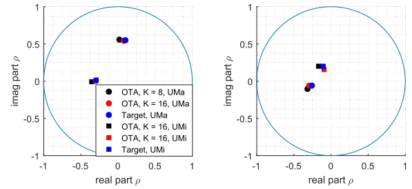
FIGURE 12. Measured antenna correlation for the target and emulated ( K = 8 and K = 16 ) channel models for the second mockup antenna in the free space mode (left) and user influence mode (right).
