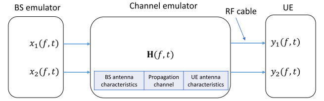
FIGURE 1. A system schematic for 2 × 2 MIMO with conducted two-stage method.
