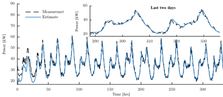
Fig. B.4: Performance of proposed estimation method throughout a 14-day period, evaluated on real consumption data.
