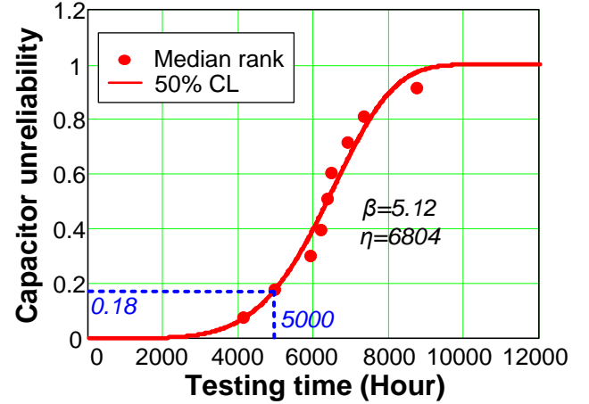
Fig. 9. Time-to-failure of capacitors at 50% Confidence Levels (CL) by using Weibull distribution using upper category temperature of 105 °C.
