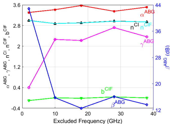
Fig. 14. Parameters of the ABG, CI, and CIF path loss models for prediction in frequency in the UMa scenario. The measurement set is for all frequencies except the excluded one shown on the x -axis which is the prediction set. Note that the scale for \beta (dB) in the ABG model is to the right.
