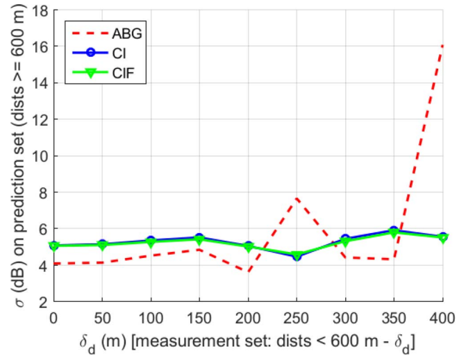
Fig. 11. SF standard deviation of the ABG, CI, and CIF path loss models for prediction in distance when the measurement set is closer to the transmitter in the UMa scenario.
