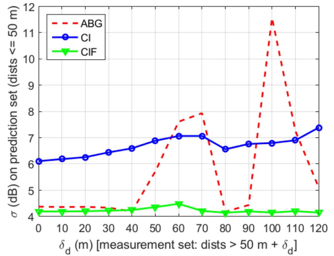
Fig. 7. SF standard deviation of the ABG, CI, and CIF path loss models for prediction in distance when the prediction set is closer to the transmitter in the UMi SC scenario.
