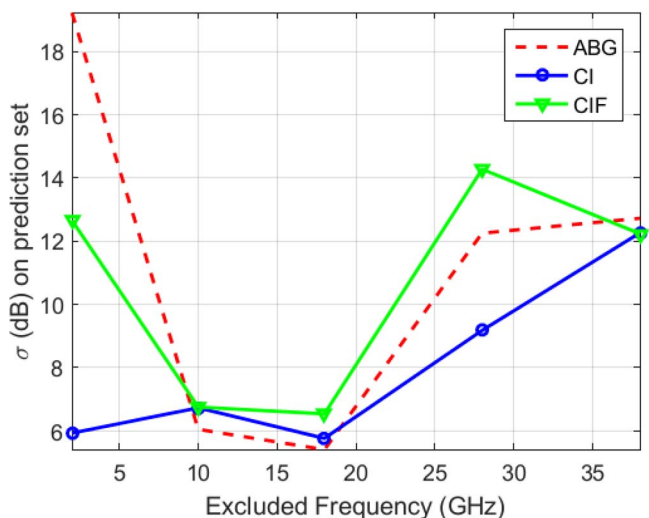
Fig. 13. SF standard deviation for the ABG, CI, and CIF path loss models for prediction in frequency in the UMa scenario. The measurement set is for all frequencies except the excluded one shown on the x -axis which is the prediction set.
