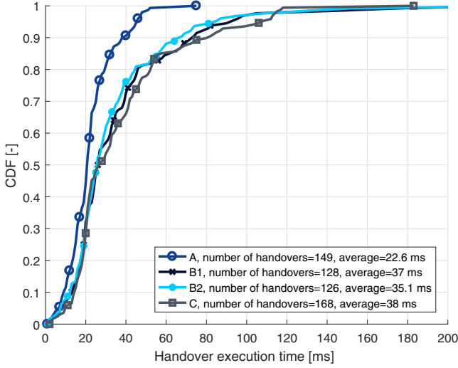
Fig. 5. Handover execution time per operator.
