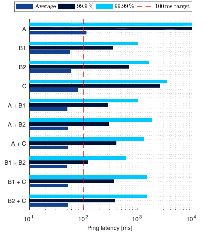
Fig. 9. Ping latency statistics for combined operator measurements.
