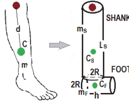
Fig. 10 – Model of the lower leg of the pendulum test.
