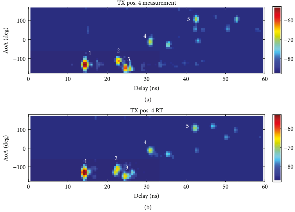
FIGURE 9: Measured (a) and RT-simulated (b) power-angle-delay profile for Tx position 4 in the basement scenario. Note that all identified multipath components are present within the 60 ns delay range in the LOS region.
