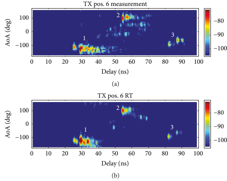
FIGURE 11: Measured (a) and RT-simulated (b) power-angle-delay profiles for Tx position 6 in the basement scenario. Note that all identified multipath components are present within the 100 ns delay range in the non-LOS region.
