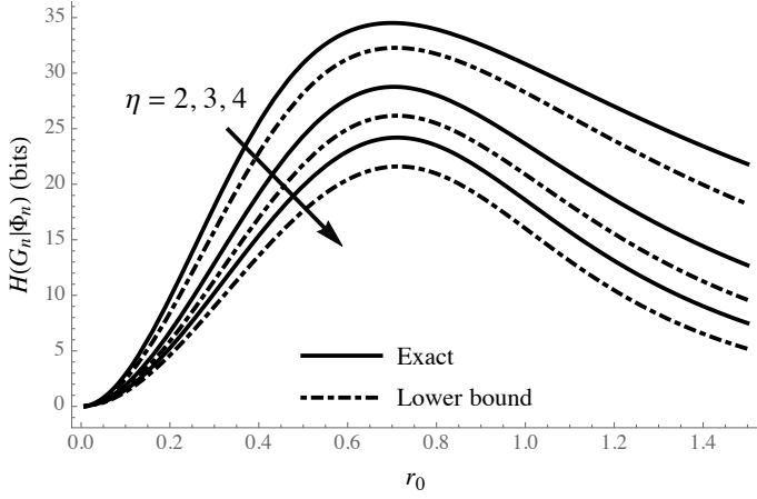
Fig. 3. Conditional entropy of a ten-node RGG with canonical wireless pair connection function in a circle of radius 1/\sqrt{\pi} ; the lower bound of Proposition 3 is shown; path loss exponent values are \eta = 2, 3, 4 .
