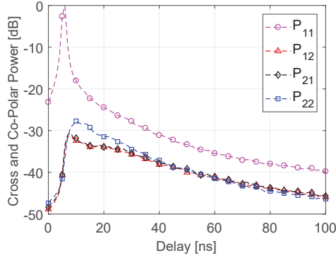
Fig. 3: PDP for 0/90° MIMO channel. Receiver at Location I.
