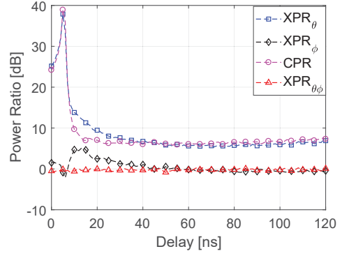
Fig. 4: Power Ratios for 0/90° MIMO channel. Receiver at Location I.
