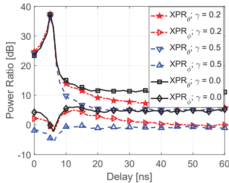
Fig. 8: Effects of mixing parameter on power ratio.
