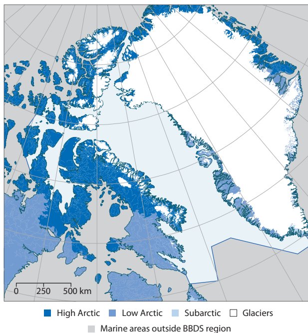
Figure 2.2 The BBDS region lies mostly within the Low Arctic and High Arctic climate zones; only a small area in South Greenland is Subarctic. Adapted from CAVM Team (2003) data set.
