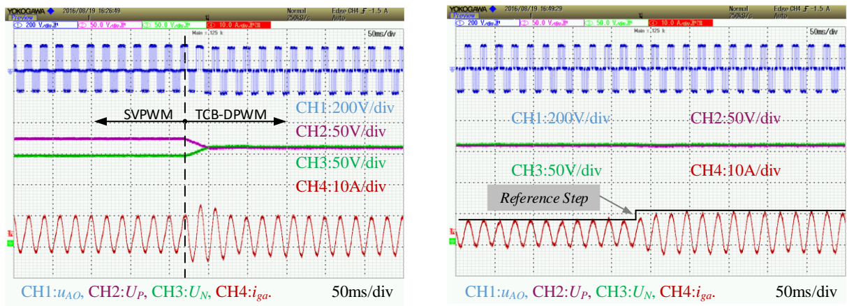
Fig.14. Experimental results neutral point voltage control at m=0.8 , \varphi=0 ( f_s=9\text{kHz} ).
