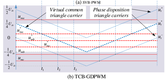
Fig.6. Relationships between SVB-PWM and TCB-PWM.
