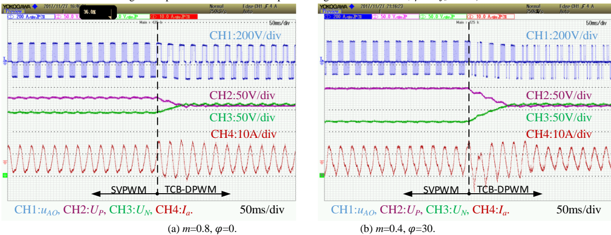
Fig.16. Experimental results neutral point voltage control at the low switching frequency ( f_s=2\text{kHz} ).
