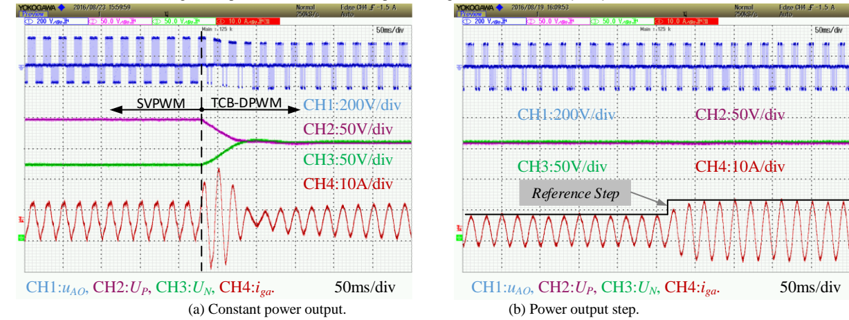
Fig.15. Experimental results neutral point voltage control at m=0.4 , \varphi=30 ( f_s=9\text{kHz} ).
