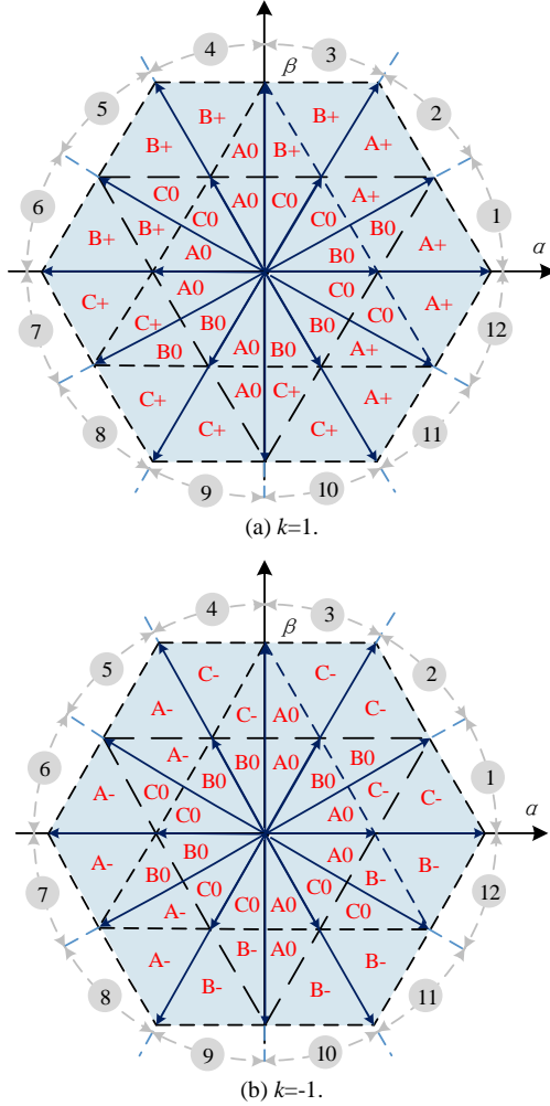
Fig.3. The clamped phases and clamped voltage levels in each sector.
