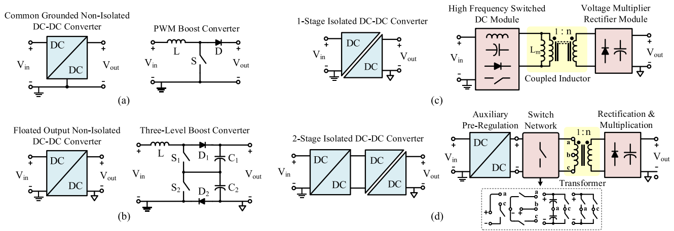
Fig. 2. Different nonisolated and isolated dc–dc converter structures. (a) Common grounded and (b) floated output nonisolated dc–dc converters. (c) Single-stage and (d) two-stage isolated dc–dc converters.
