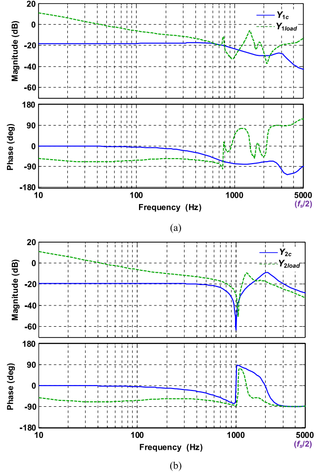
Fig. 16. Frequency responses of the control output admittances, Y_{1c}(s) and Y_{2c}(s) , and the equivalent system admittances, Y_{1load}(s) and Y_{2load}(s) , after using the damping controllers. (a) Converter-side current control. (b) Grid-side current control.
