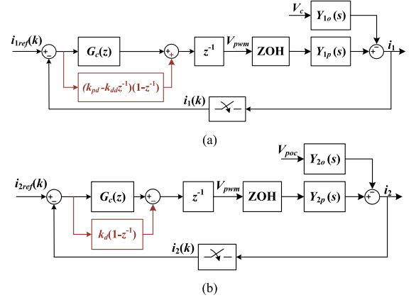
Fig. 10. Block diagrams of the proposed damping control methods. (a) Converter-side current control. (b) Grid-side current control.
