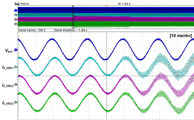
Fig. 23. Measured PCC (line-to-line) voltage, and the phase-A grid currents of three paralleled VSCs with the grid-side current control. i_2 : [5 A/div]. V_{pcc} : [500 V/div].
