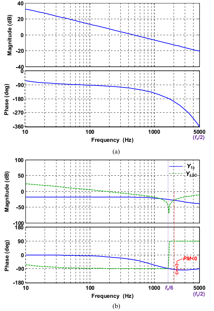
Fig. 5. Frequency responses of converter-side current control. (a) Open-loop gain T_1(s) . (b) Control output admittance Y_{1c}(s) and the admittance Y_{L2C}(s) .
