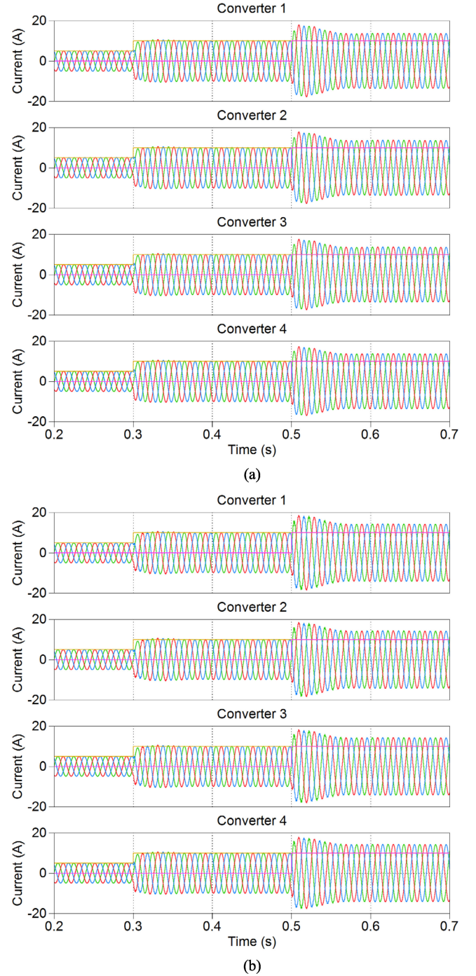
Fig. 18. Simulated step responses of grid-side currents of four paralleled VSCs with the damping controller included. (a) Converter-side current control. (b) Grid-side current control.
