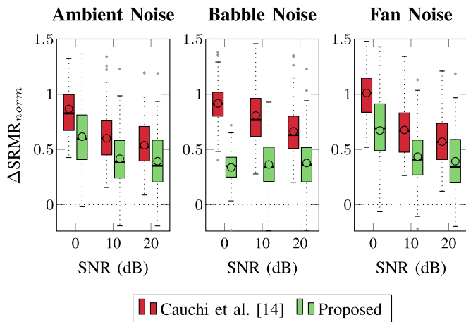
Fig. 10. Differential SRMR_{norm} scores for different noise conditions, averaged across all acoustic scenarios.
