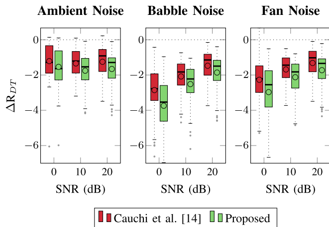
Fig. 9. Differential R_{DT} scores obtained for different noise conditions, averaged across all acoustic scenarios.
