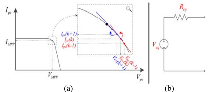
Fig. 5. (a) Extrapolation of the predicted PV current based on the predicted PV voltage and the straight line equation, (b) PV module equivalent circuit model used for the prediction of the PV string power.
