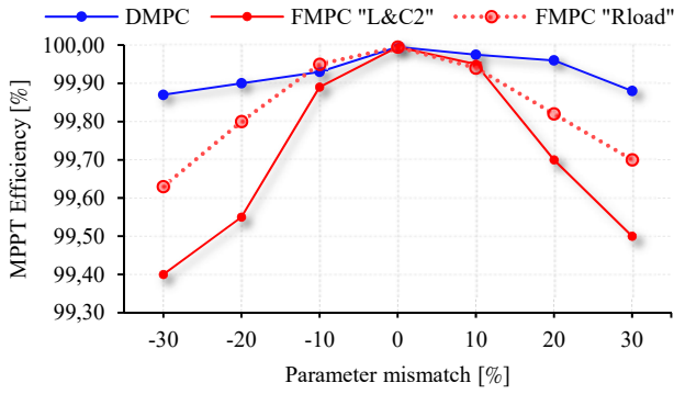
Fig. 17. Experimental results of FMPC-MPPT and DMPC-MPPT efficiencies under STC in case of model parameter mismatch “L and C 2 ”. The red dash line represents FMPC efficiencies with load value misestimated “R load ”.
