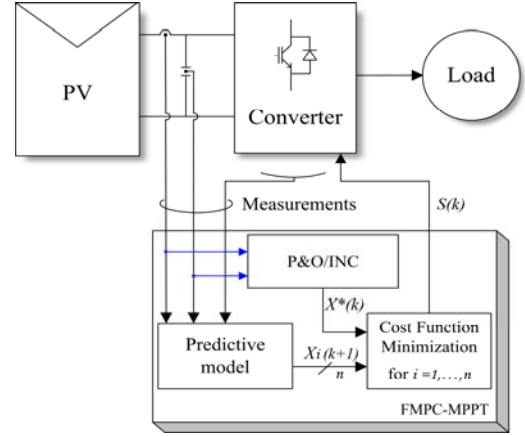
Fig. 2. General control block diagram of FMPC used for tracking the MPP.
