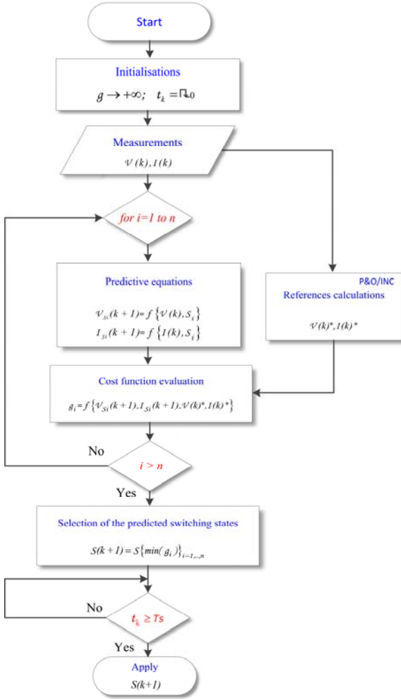
Fig. 4. A Flowchart of the general Finite control set MPC-based MPPT.
