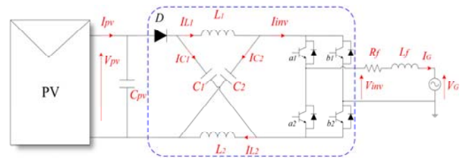
Fig. 8. Simplified schematic of the overall grid connected PV system configuration using Z-source inverter.
