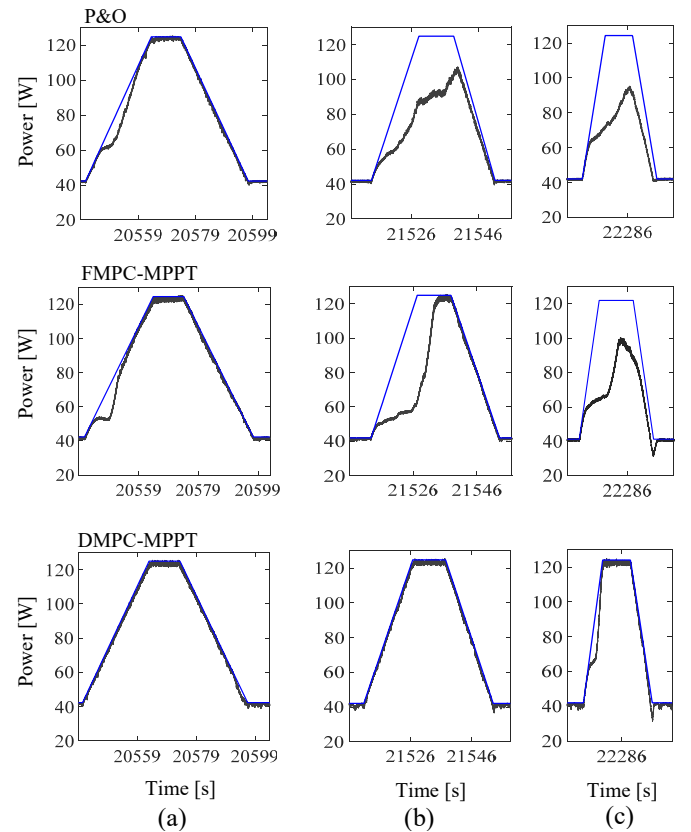
Fig. 16. Experimental results of P&O, FMPC-MPPT, and DMPC-MPPT, respectively, under low to high irradiance EN50530 standard test “30% - 100%”: (a) one repetition from the sequence before the last two sequences “30W/m 2 /s”, (b) one repetition from the one before the last sequence “50W/m 2 /s”, and (c) one repetition from the last sequence “100W/m 2 /s”.
