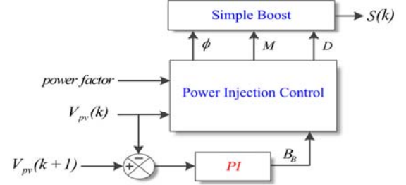
Fig. 10. The overall procedure of defining the switching state based on the predicted PV voltage, and the desired power factor.
