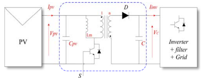
Fig. 11. Simplified schematic of the overall grid connected PV system configuration using flyback converter as an interface for tracking the MPP.
