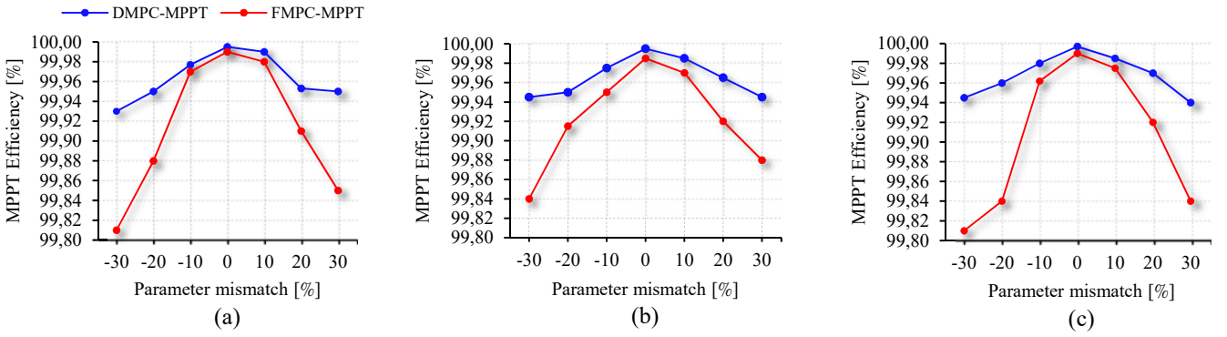
Fig. 14. Simulation results of FMPC-MPPT and DMPC-MPPT efficiencies under STC, and in case of model parameter mismatch using: (a) Boost converter “ L and C_2 ”, (b) Z-source inverter “ C_l and L_l ”, and (c) Flyback converter “ C and L_m ”.
