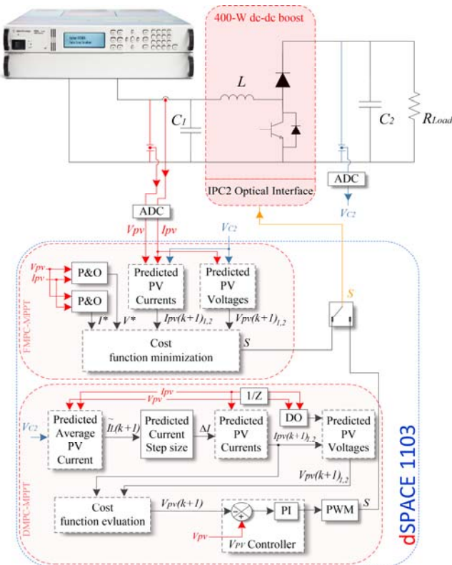
Fig. 12. Global diagram of the experimental test bench, and the main control structure of both discrete MPC-MPPT methods using boost converter.
