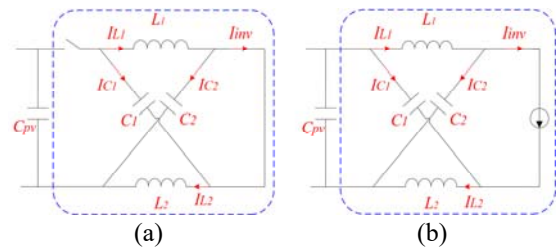
Fig. 9. (a) ZSI equivalent circuit in a Shoot-Through state, (b) ZSI equivalent circuit in a Non-Shoot-Through state.
