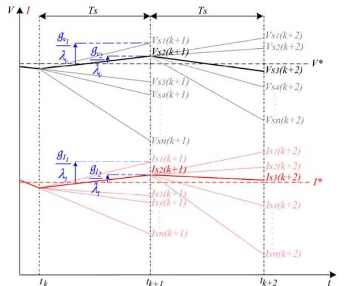
Fig. 3. The operation principle of a FMPC method on power electronics.
