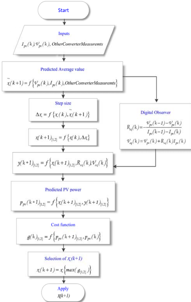
Fig. 6. A Flowchart of the general DMPC-MPPT.
