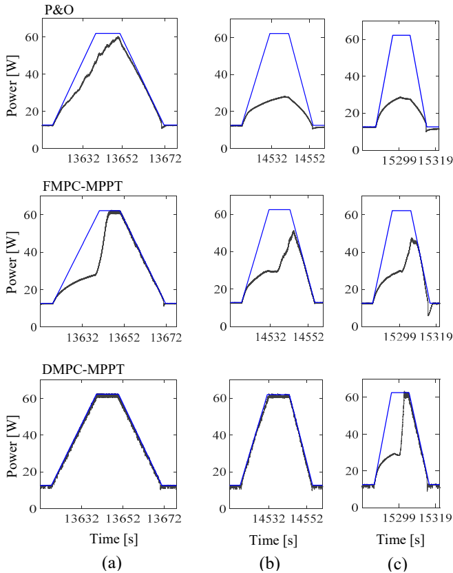
Fig. 15. Experimental results of P&O, FMPC-MPPT, and DMPC-MPPT, respectively, under very low to medium irradiance EN50530 standard test “10% - 50%”: (a) one repetition from the sequence before the last two sequences “20W/m 2 /s”, (b) one repetition from the one before the last sequence “30W/m 2 /s”, and (c) one repetition from the last sequence “50W/m 2 /s”.
