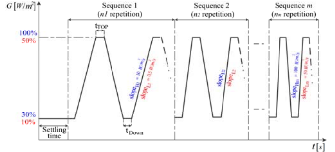
Fig. 13. The irradiance profiles used to calculate the dynamic efficiency of the MPPT, according to EN 50530 standard. The red and blue colors indicate to the solar irradiation ranges and slopes of very low to medium irradiance test and low to high solar irradiance test, respectively.
