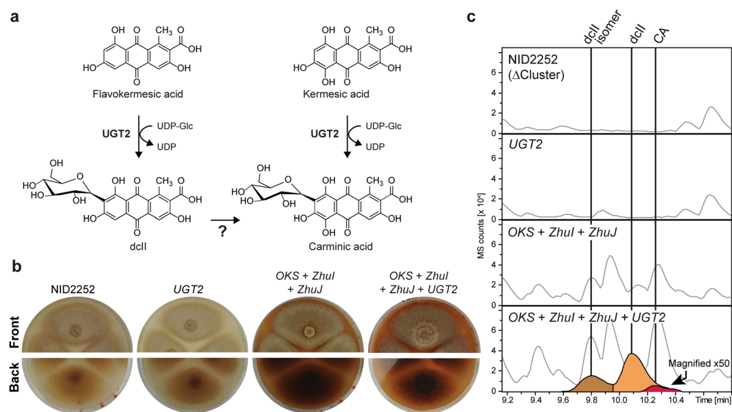
Figure 5. Glucosylation step for forming carminic acid. (a) The Dactylopius coccus glucosyltransferase UGT2 accepts both kermesic acid and flavokermesic acid as substrates, resulting in the formation of carminic acid and dcII, respectively. (b) The phenotypic effect of expressing UGT2 alone and in combination with the synthetic PKS in the NID2252 Aspergillus nidulans background, pictures taken after seven days of incubation. (c) Targeted metabolic analysis for the production of glucosylated compounds, e.g. carminic acid (red) and dcII (orange) overlaid base peak chromatogram (light grey).
