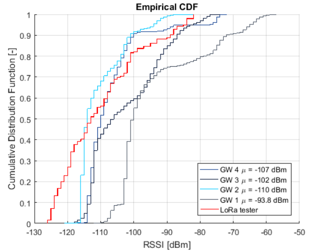
Fig. 6. RSSI for all received packets per gateway.
