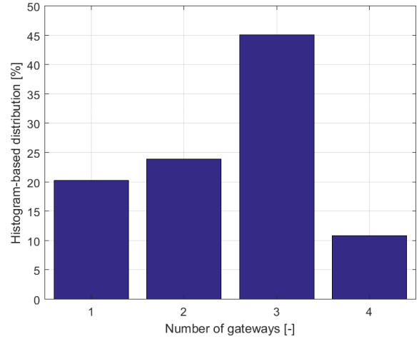
Fig. 5. Average number of gateways receiving a packet from a node.
