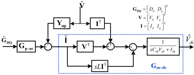
Fig. 4. Small-signal model of dc-link dynamics G_{p-dc} .
