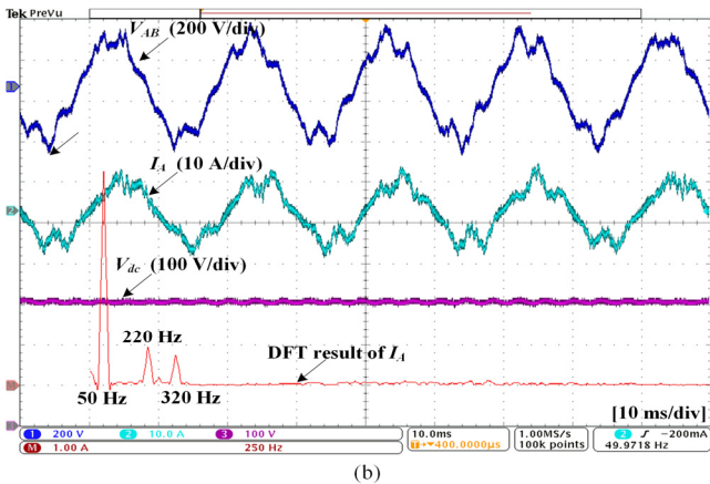
Fig. 19. Experimental waveforms of the PCC voltage, input current and dc-link voltage in the rectifier mode. (a) k_p=0.5 . (b) k_p=1.4 .
