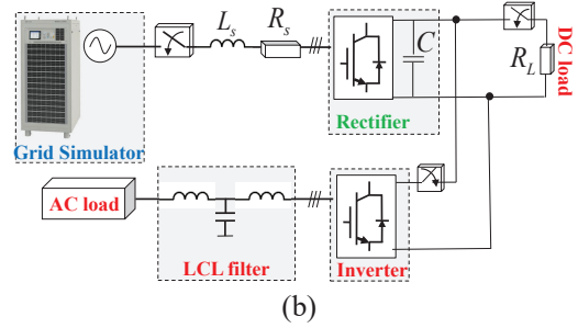
Fig. 5. (a) Experimental setup, (b) system architecture.
