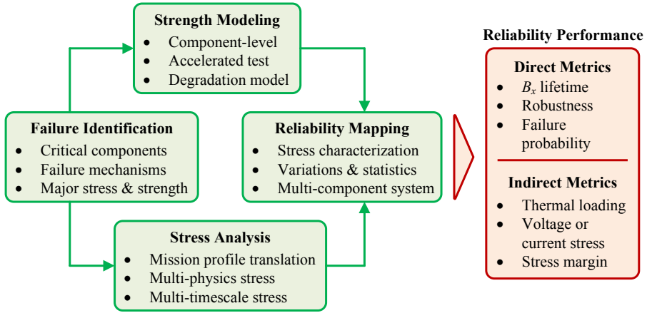
Fig. 1.5: Design for Reliability (DfR) flow diagram for power electronics converters, which can be employed to assess the reliability performance of the designed PV inverter [39].
