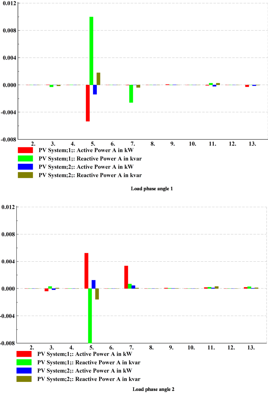
Fig. 4: Injected active and reactive power
