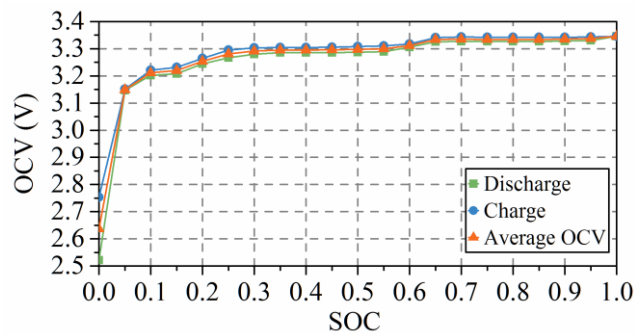
Figure 7. OCV measurement.
