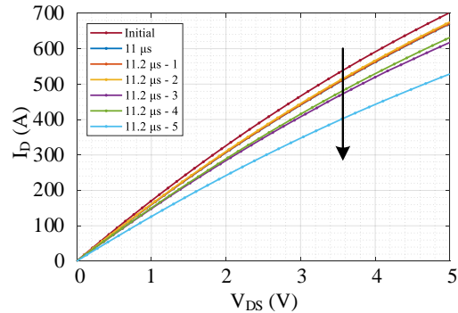
Fig. 10. On-state resistance increases after repetitive SC tests at 11.2 \mu\text{s} ( V_{GS}=20\text{V} ).
