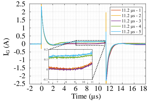
Fig. 6. Calculated gate current ( I_G ) waveforms from the first to fifth repetitive SC test at 11.2 \mu\text{s} ( V_{DS}=500\text{V} ).
