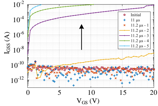
Fig. 8. Gate leakage current increases after repetitive SC tests at 11.2 \mu\text{s} .
