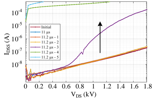
Fig. 9. Drain leakage current increases after repetitive SC tests at 11.2 \mu\text{s} .
