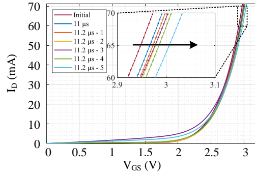
Fig. 7. Threshold voltage shifts after repetitive SC tests at 11.2 \mu\text{s} ( V_{DS}=20\text{V} ).
