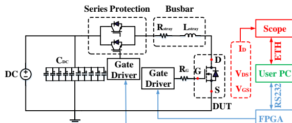
Fig. 1. Principle schematic of the Non-Destructive Tester (NDT).
