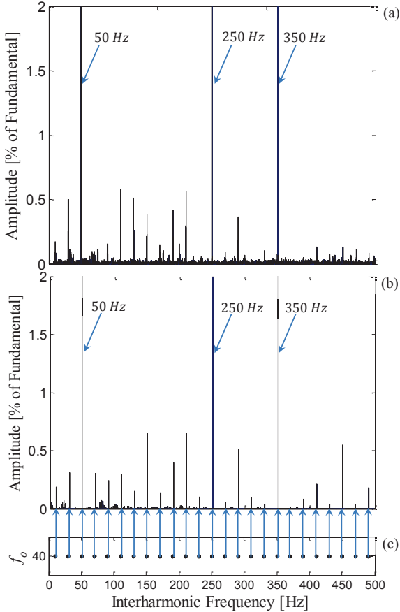
Fig. 12. Drive input current i_a interharmonics at the output frequency f_o = 40 Hz and load torque T_L = 12 Nm by applying an asymmetrical regularly sampled SVM modulation technique: (a) Experimental result, (b) Simulation result, and (c) Output frequency versus interharmonic frequencies.
