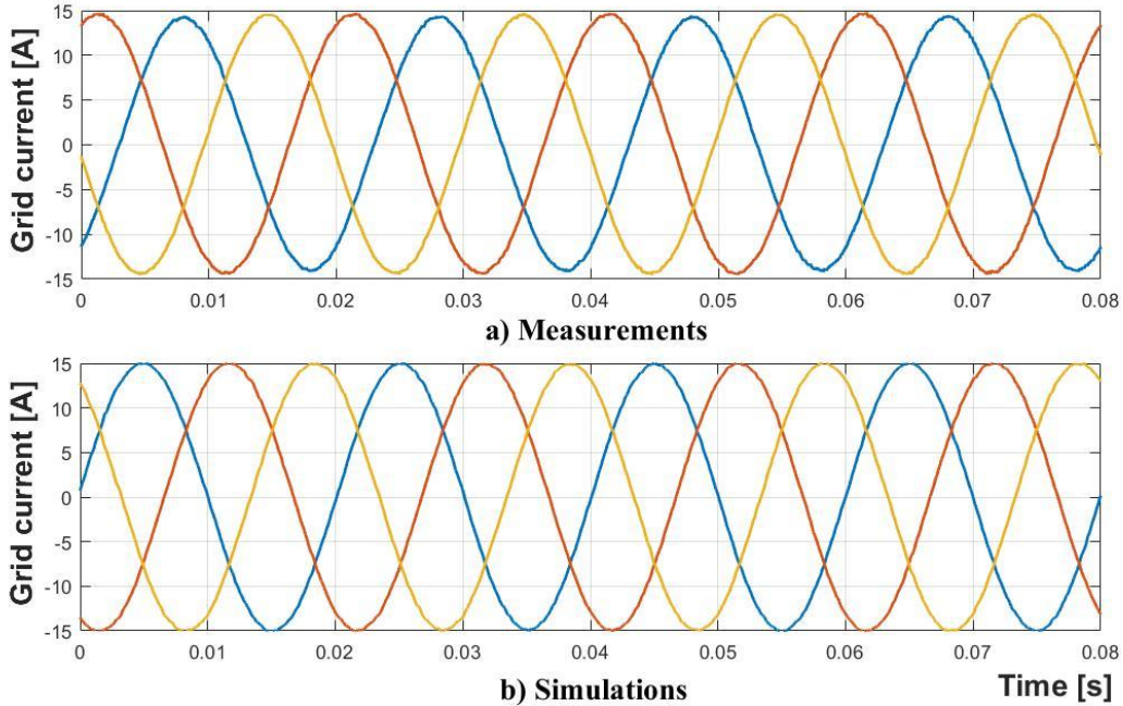
Fig. 5: Steady state results from a) experiments with \text{THDi} = 1.08\% and b) simulations with \text{THDi} = 1.62\% . Both results are with K_p = 30 and K_i = 800 .
