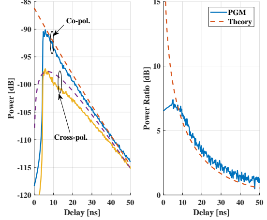
Fig. 3: Polarimetric power and power ratio from propagation graph and approximate expressions.
