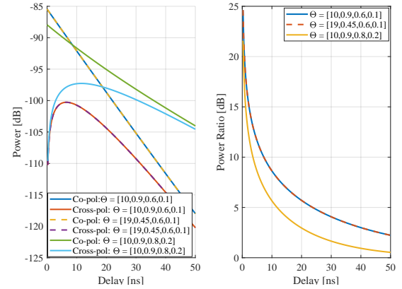
Fig. 4: Polarimetric power and power ratio with different parameters. \Theta denotes the parameter set [N_s, P_{\text{vis}}, g, \gamma] .
