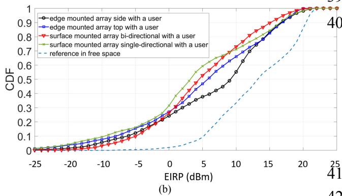
FIGURE 14. (a) User body blockage for the antenna arrays with four element designs (within the red line). (b) The spherical coverage with user body blockage for the antenna arrays. (total accepted power = 10 dBm).
