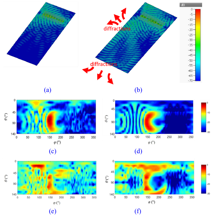
FIGURE 9. Normalized current distribution for an 8x1 array in a mobile phone size chassis (a) without the glass back cover and (b) with the glass back cover when the array pattern is steered to 60° bias from the bore-sight of the ground plane at 28 GHz. Comparison of the corresponding (c) measured and (d) simulated radiation pattern without the glass back cover. Comparison of the corresponding (e) measured and (f) simulated radiation pattern with the glass back cover.
