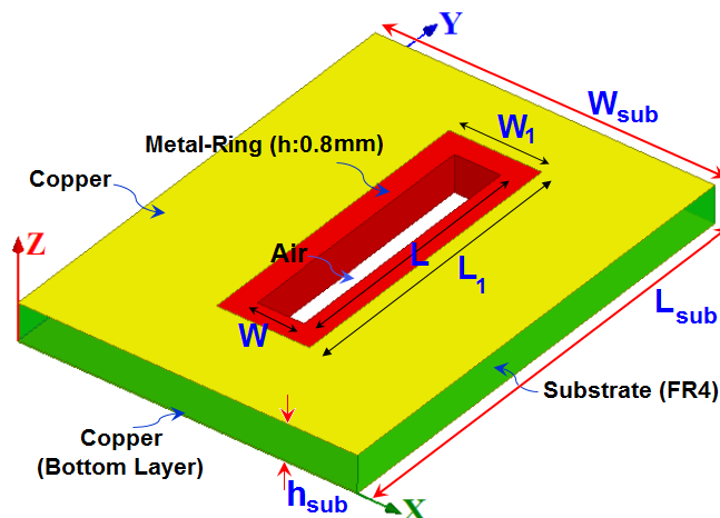
Fig. 1. Geometry of the proposed insensitive slot-loop antenna.
