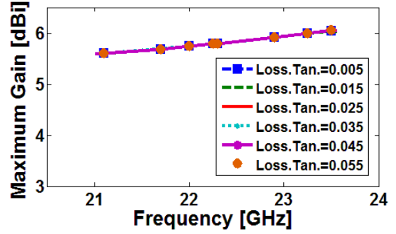
Fig. 8. Simulated maximum gain characteristics of the proposed antenna for different values of loss tangent.
