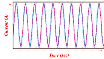
Fig. 25. Experimental grid current injected to the utility grid at unity PF operation with proposed (red line) and conventional controllers (blue line).
