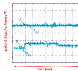
Fig. 32. Power capability of proposed control system.
