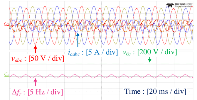
Fig. 16. Steady-state experimental results of the power converter with the conventional virtual inertia control ( v_{abc} : the grid voltages, i_{cabc} : the converter currents, v_{dc} : the DC-link voltage, and \Delta f_r : the frequency change).
