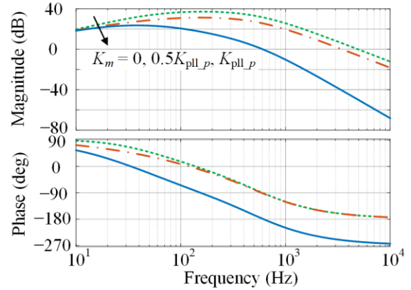
Fig. 13. Bode diagram of G_{id\_ \Delta v_{ref\_wp}}(s) , i.e., the transfer function from i_{cd} to \Delta v_{dc\_ref} with the proposed virtual inertia control.
