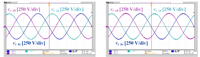
(a) Three phase capacitor voltage v_{c\ abc} for R_{load} ( 48\Omega ), Voltage THD: 1.15%.
