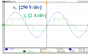
(c) Capacitor voltage v_{c\ ab} and load current i_{o\ a} for non-linear load, Voltage THD: 1.35%.
