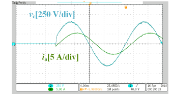
(d) Capacitor voltage v_{c\ ab} and load current i_{o\ a} for step change with R_{load} .
