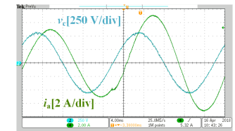
(f) Capacitor voltage and load current v_{c\ ab} and i_{o\ a} for a step load change (linear RL_{load} , R_{load} = 48 \rightarrow 34\Omega ).
