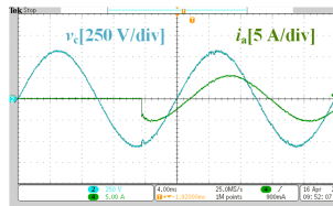
(e) Capacitor voltage and load current v_{c\ ab} and i_{o\ a} for a step load change (linear R_{load} = 0 \rightarrow 48\Omega ).
