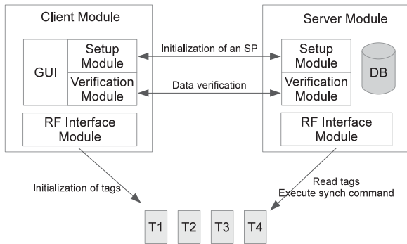
Fig. 12. Program modules of the client and server.
