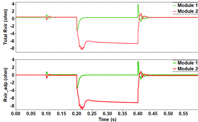
Fig. 25. The adaptive virtual impedance and the total virtual impedance of the two modules in one phase.
