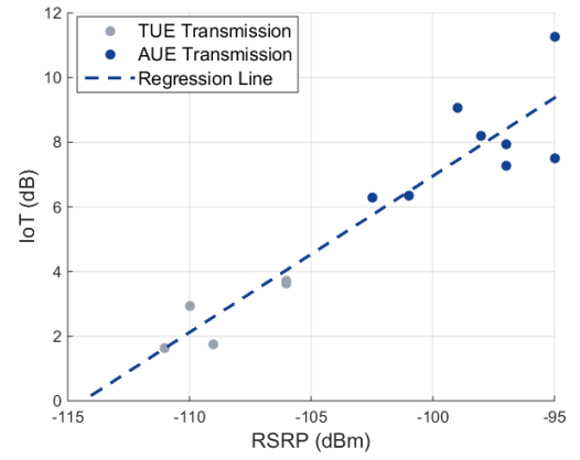
Fig. 4. IoT versus downlink reference symbol received power (RSRP) from neighbor cells.
