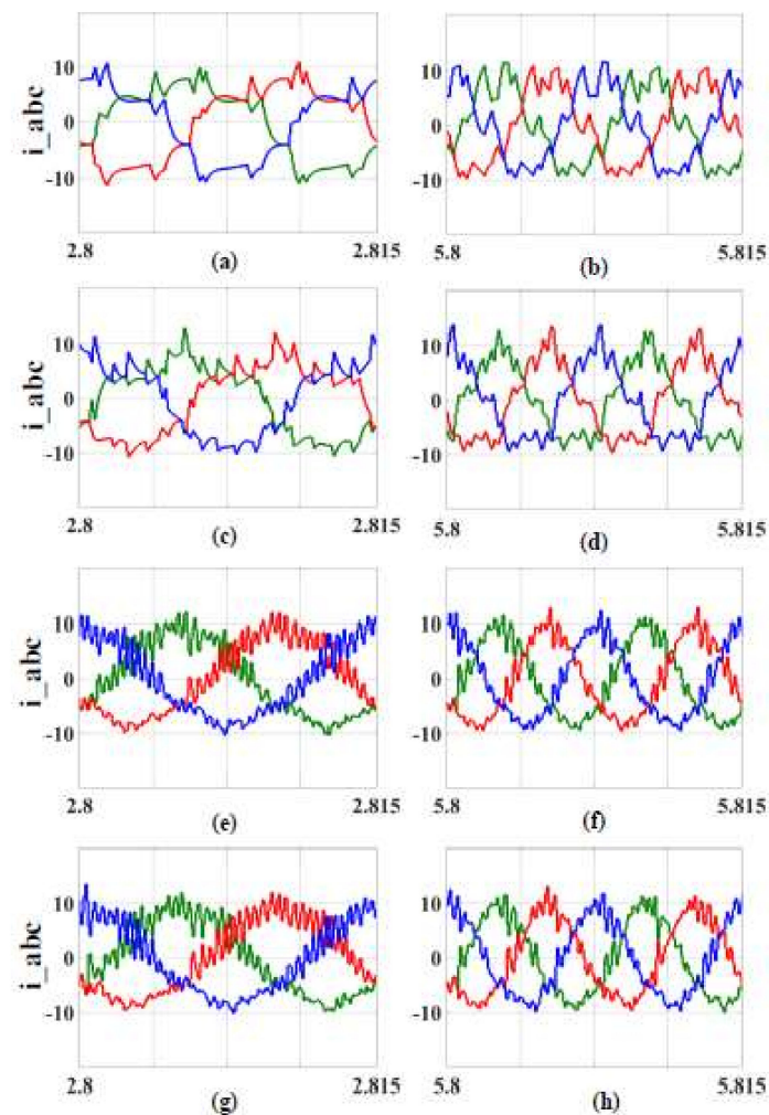
Figure 12. Motor current waveforms. (a) wOVPIwO3D at TP1. (b) wOVPIwO3D at TP2. (c) wVPIwO3D at TP1. (d) wVPIwO3D at TP2. (e) wVPIw3D at TP1. (f) wVPIw3D at TP2. (g) stiffwVPIw3D at TP1. (h) stiffwVPIw3D at TP2.
