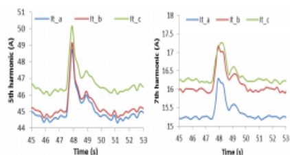
(a) Transient 5 th and 7 th harmonics of bow thruster current (AC bus quasi-balanced voltage UF=0.35%)
