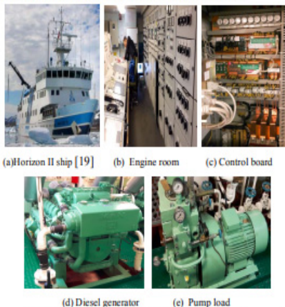
Fig.2 Horizon-II research training ship test environment
