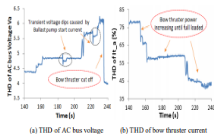
Fig.12 THD of the AC bus voltage and bow thruster current
