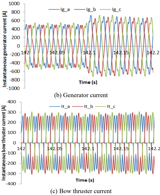
Fig.3.5. Instantaneous values examples considering the voltage dip
