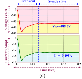
Fig. 7. Numerical Computing Matrix Laboratory 9.0 (R2016a) Simulation Result of proposed 2LC_m -Y converter with 10V, 240W, 0.60 duty cycle with 50kHz switching Frequency (a) 2LC_m -2LVD converter output current and voltage (b) 2LC_m -2LCVD converter output current and voltage (c) 2LC_m - 2LC_m VD converter output current and voltage.
