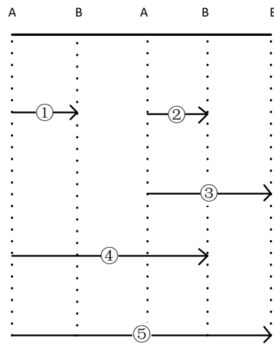
Figure 2. Effective sequences A \rightarrow B under different max\_win conditions.
