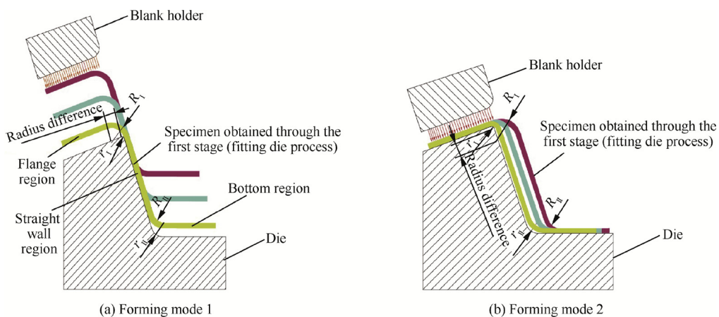
Fig. 5 Forming modes of rounded corner radii from big values to small ones in the second stage.
