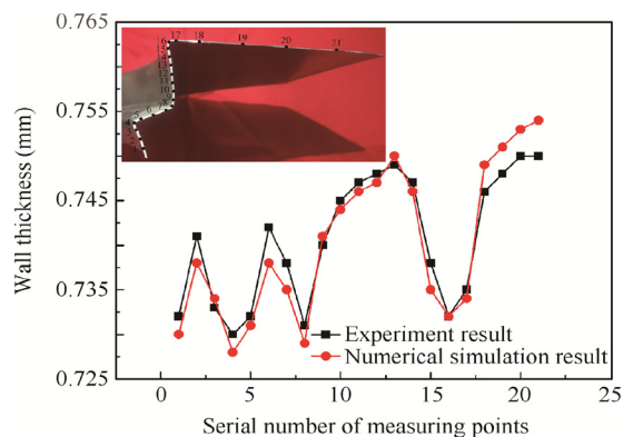
Fig. 21 Comparison of thickness distributions between experiments and FEM.
