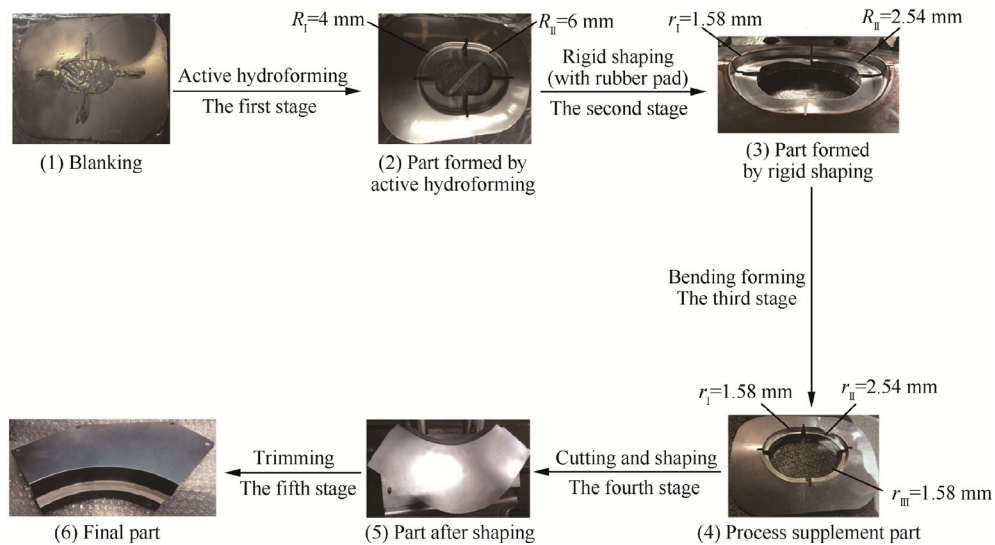
Fig. 4 Manufacturing process of the irregular complex part.
