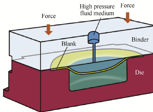
Fig. 2 Principle drawing of HPFMF.
