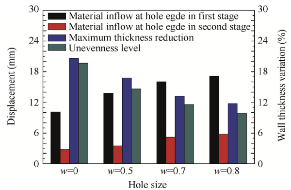
Fig. 16 Material inflow volume and wall thickness variation with different values of w .
