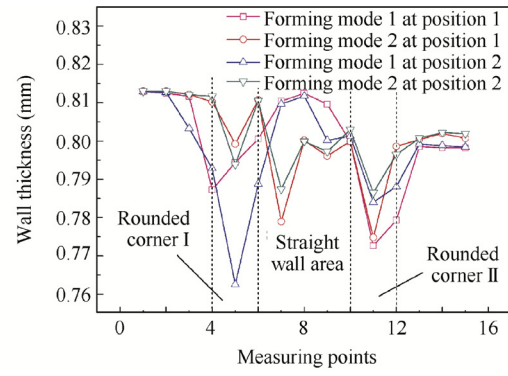
(b) Wall thickness distributions
