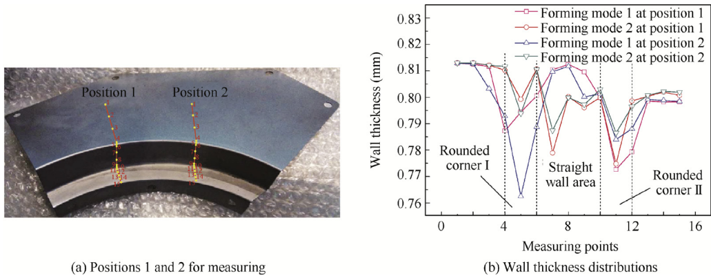
Fig. 8 Effects of forming modes on wall thicknesses.
