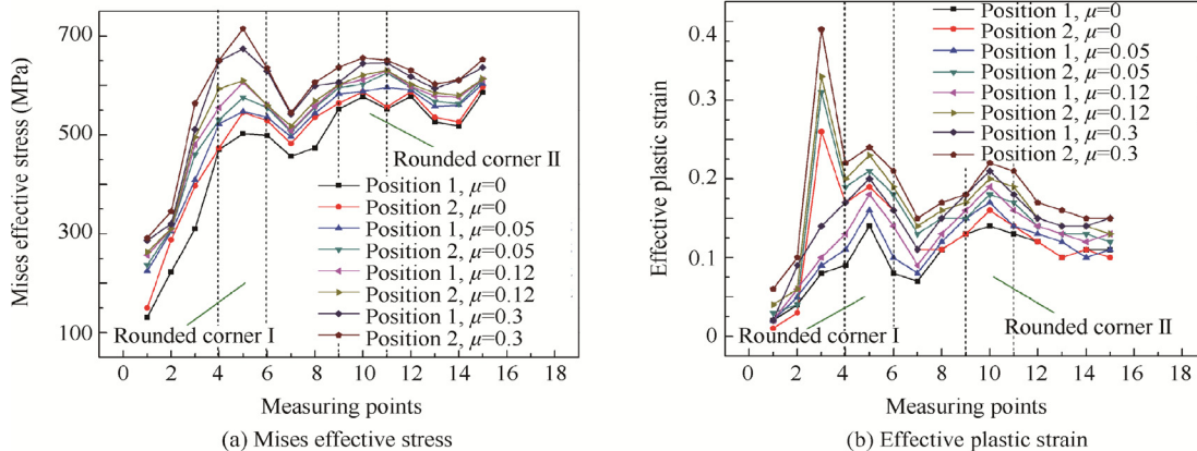
Fig. 19 Mises effective stress and effective plastic strain distributions under different friction coefficients.
