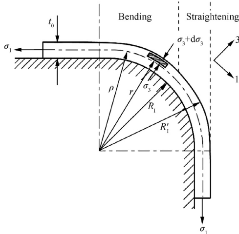
Fig. 10 Bending process of rounded corner R_1 .
