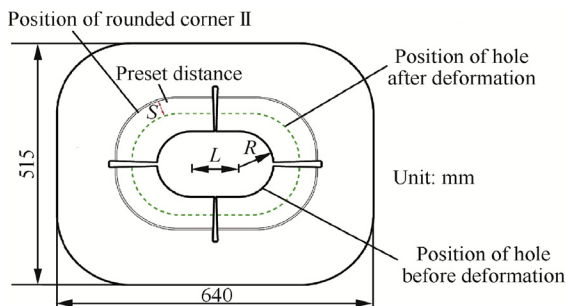
Fig. 15 Shape and dimension design for the hole.
