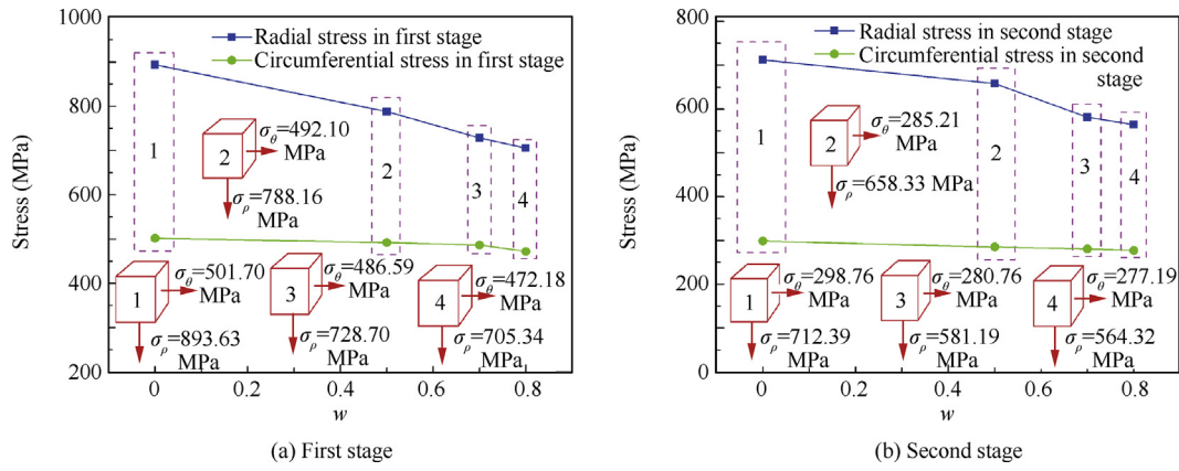
Fig. 17 Stress states in the rounded corner II region under different values of w .
