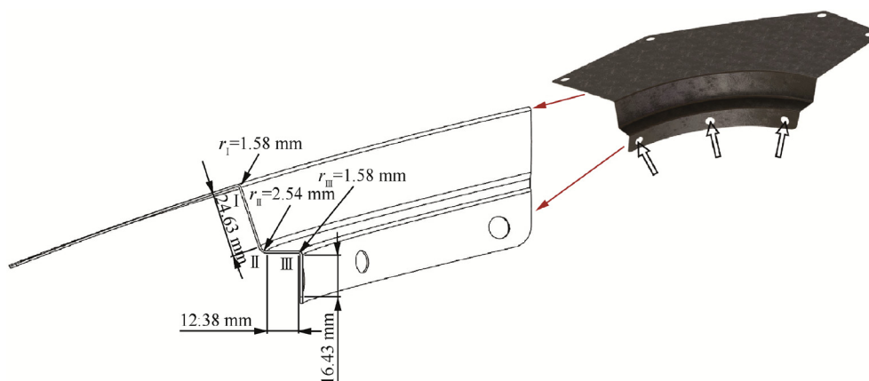
Fig. 1 Typical part with a shape and key dimensions.
