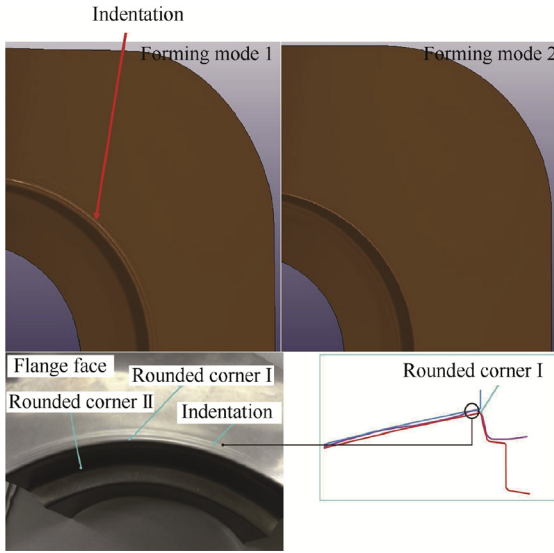
Fig. 6 Defect in the flange region produced by using forming mode one.
