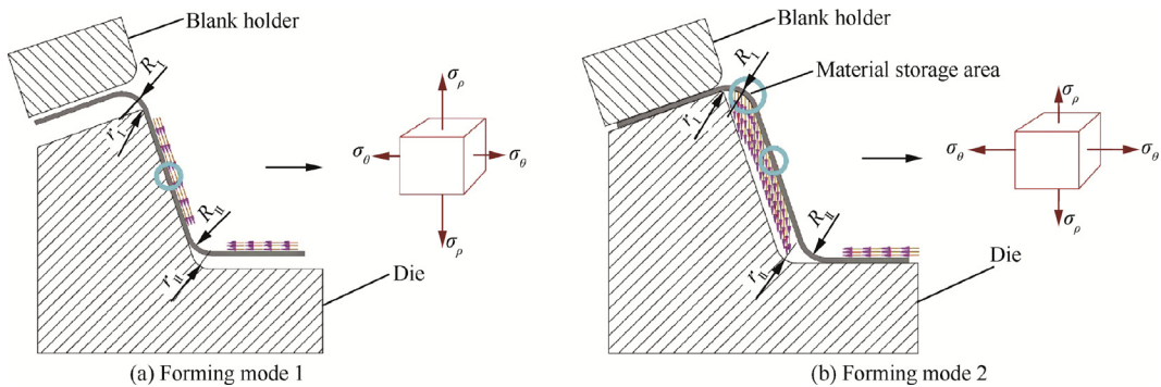
Fig. 7 Stress states of the straight wall region and material feed modes to form rounded corner r_{II} .
