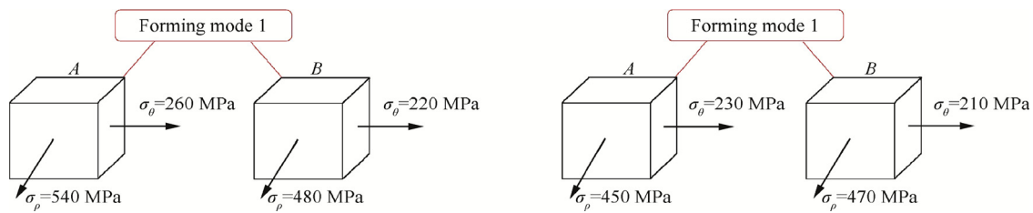
Fig. 13 Stress states at points A and B after forming.
