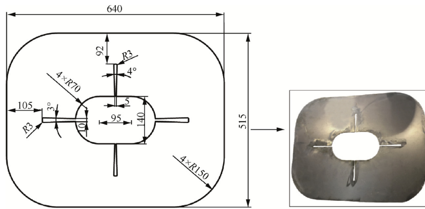
Fig. 3 Preliminary blank shape and size.
