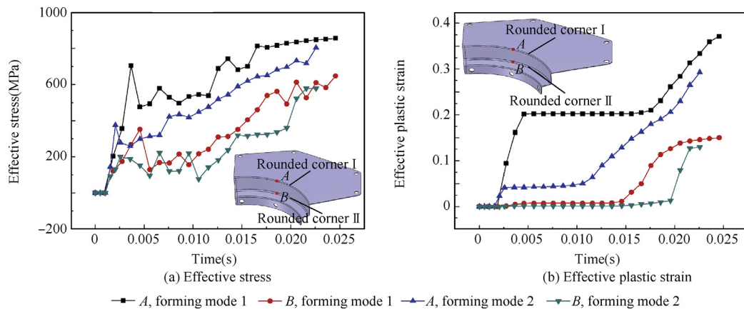
Fig. 12 Effective stress and strain evolutions at points A and B .
