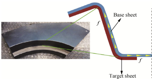
Fig. 18 Tangential friction force.
