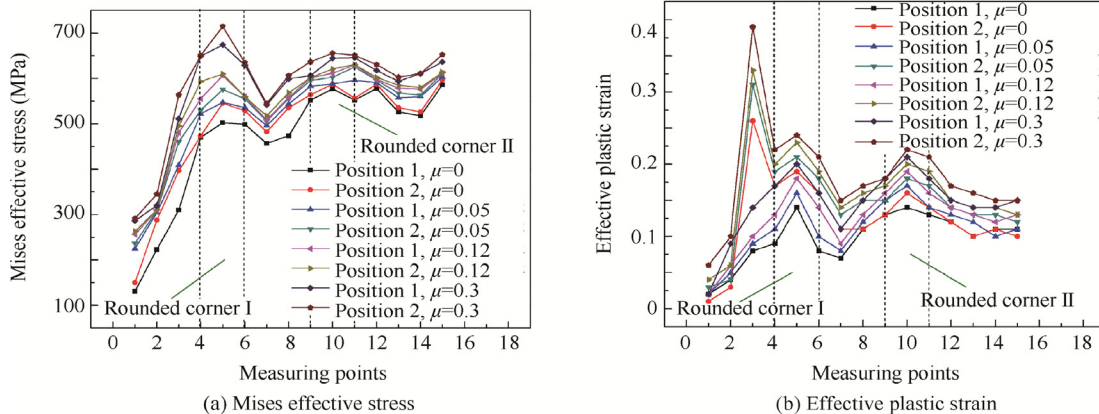
Fig. 19 Mises effective stress and effective plastic strain distributions under different friction coefficients.
