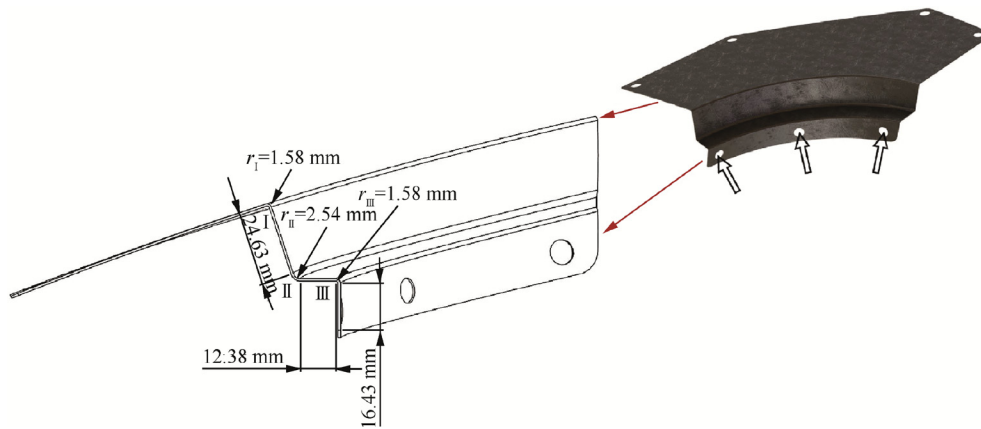
Fig. 1 Typical part with a shape and key dimensions.
