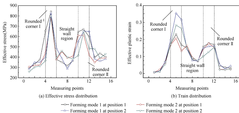
Fig. 11 Effective stress and strain distributions of the specimen at different positions.
