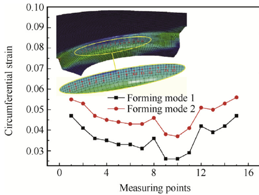
Fig. 9 Circumferential strain distribution in the straight wall region with different forming modes.
