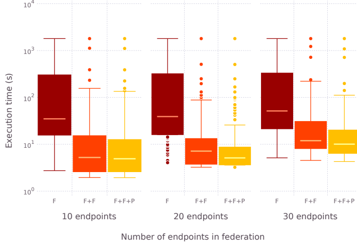
Fig. 4: Average execution time with FEDX (F), FEDX + FEDRA (F+F) and FEDX + FEDRA + PENLOOP (F+F+P).
