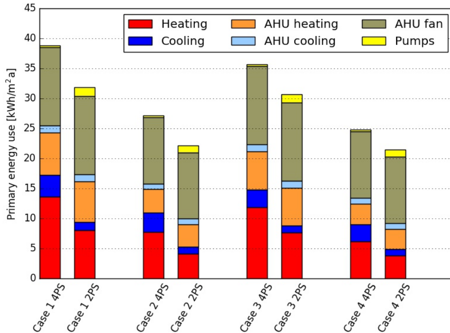
Fig. 12 Total annual primary energy use – Real configuration
