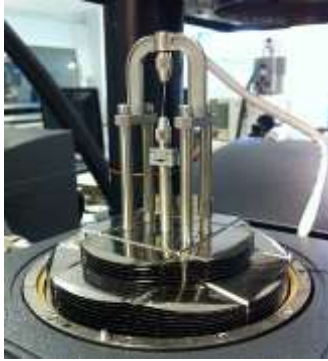
Fig. 8. Experimental setup in DMA Q800.
