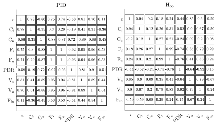
Figure A2. Correlation matrix of system parameters for the 2080–2550 s time period, with respect to the PID and H_\infty control solution. Here shown with numerical values.
