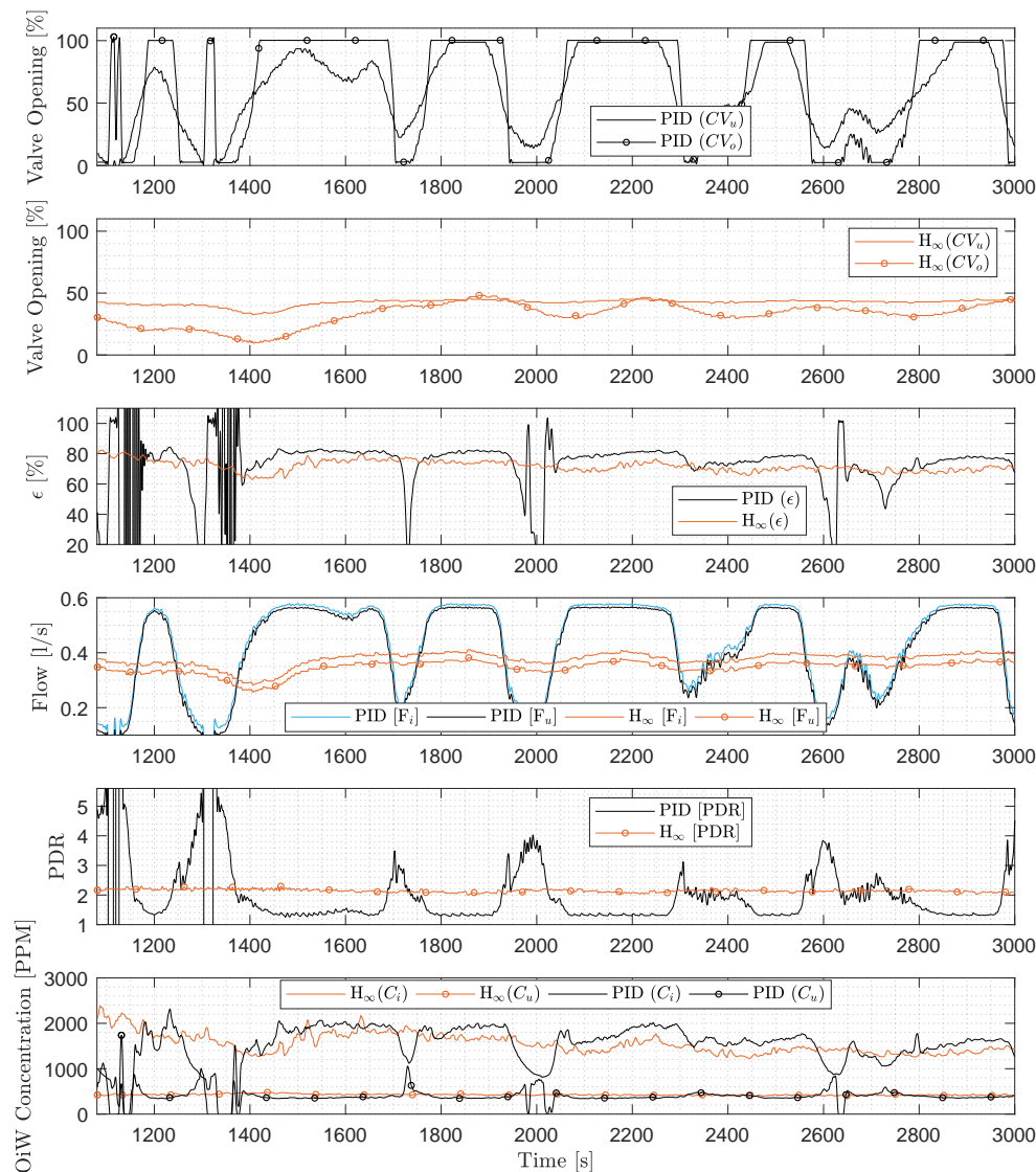
Figure 4. Experiment Results: controller evaluation with fluctuating inlet flow rate F_i . The plots show valve openings, efficiencies, flows, PDRs, and OiW concentrations.
