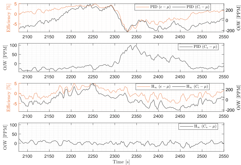
Figure 5. Experiment Results: controller evaluation with fluctuating flow rate, zoomed in on a portion of the experiment to show the dynamics of the OiW measurements. The mean has been subtracted to emphasize the dynamic relationship.
