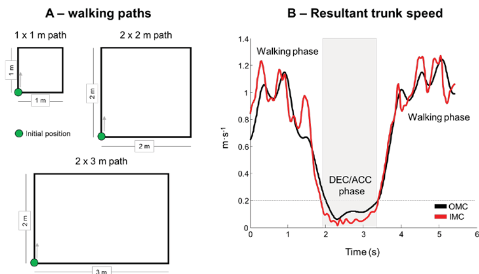
Figure 1 In A, illustrative representation of the walking paths marked on the floor of a motion capture laboratory. In B, illustrative curves from OMC and IMC during an illustrative trial.
