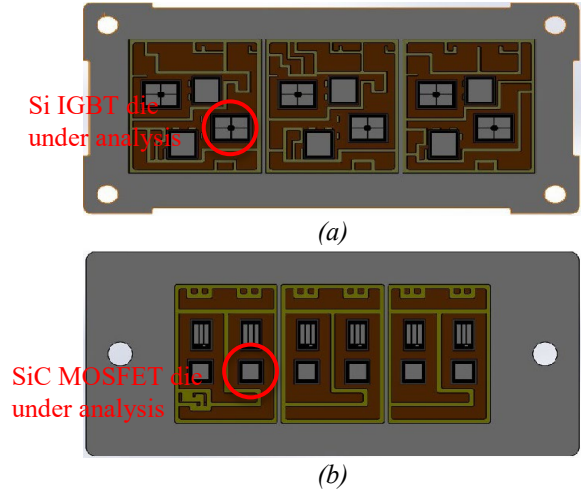
Figure 5: Modules' models (a) Si IGBT (b) SiC MOSFET
