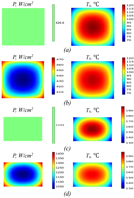
Figure 8: Top surface distribution of steady-state power density, \rho_P(x, y) , and temperature, T_s(x, y) , for a total heat of 300 W, h_{tc} = 100,000 W/(m^2 \cdot K) , and T_a = 25^\circ C : (a) Si IGBT uniform heat dissipation, (b) Si IGBT non-uniform heat dissipation, (c) SiC MOSFET uniform heat dissipation, (d) SiC MOSFET non-uniform heat dissipation'
