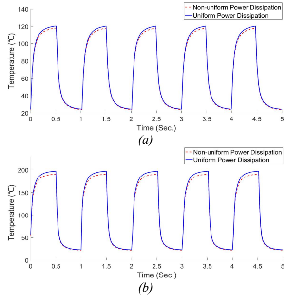
Figure 9: Transient temperature at 300 W for different power dissipations (a) Si IGBT (b) SiC MOSFET
